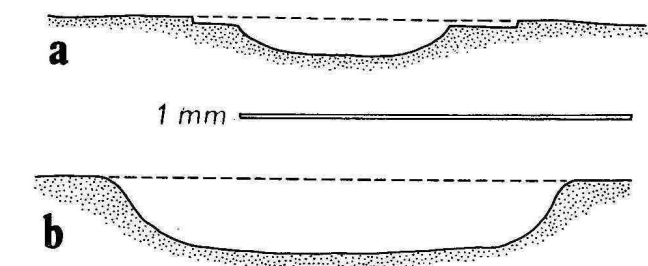
FIGURE 3. Typical cross-sections of (a) an engraved groove on the Patne ostrich eggshell object, depicting the splintering of the surface layer; and (b) a groove produced by root action, as it appears on both Indian ostrich eggshell and Siberian mammoth ivory.
