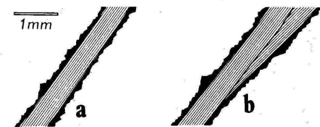
FIGURE 2. Typical engraved groove on the Patne ostrich eggshell object, with the splintering scars shown in black on either side of the groove (a); (b) depicts duplication of a groove.
